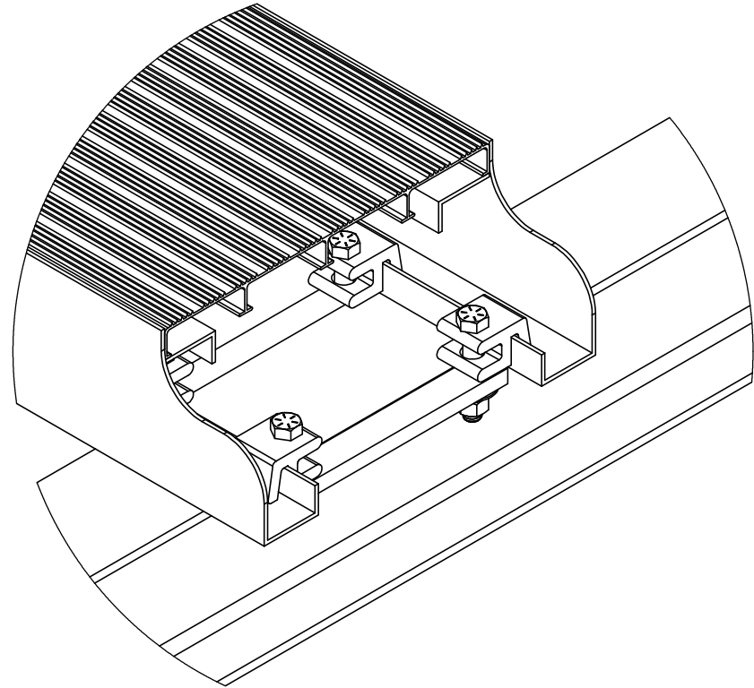
WALKBOARD CUT BACK TO SHOW MOUNT
